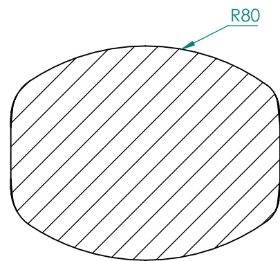
SECTION E-E SCALE 1 : 2
